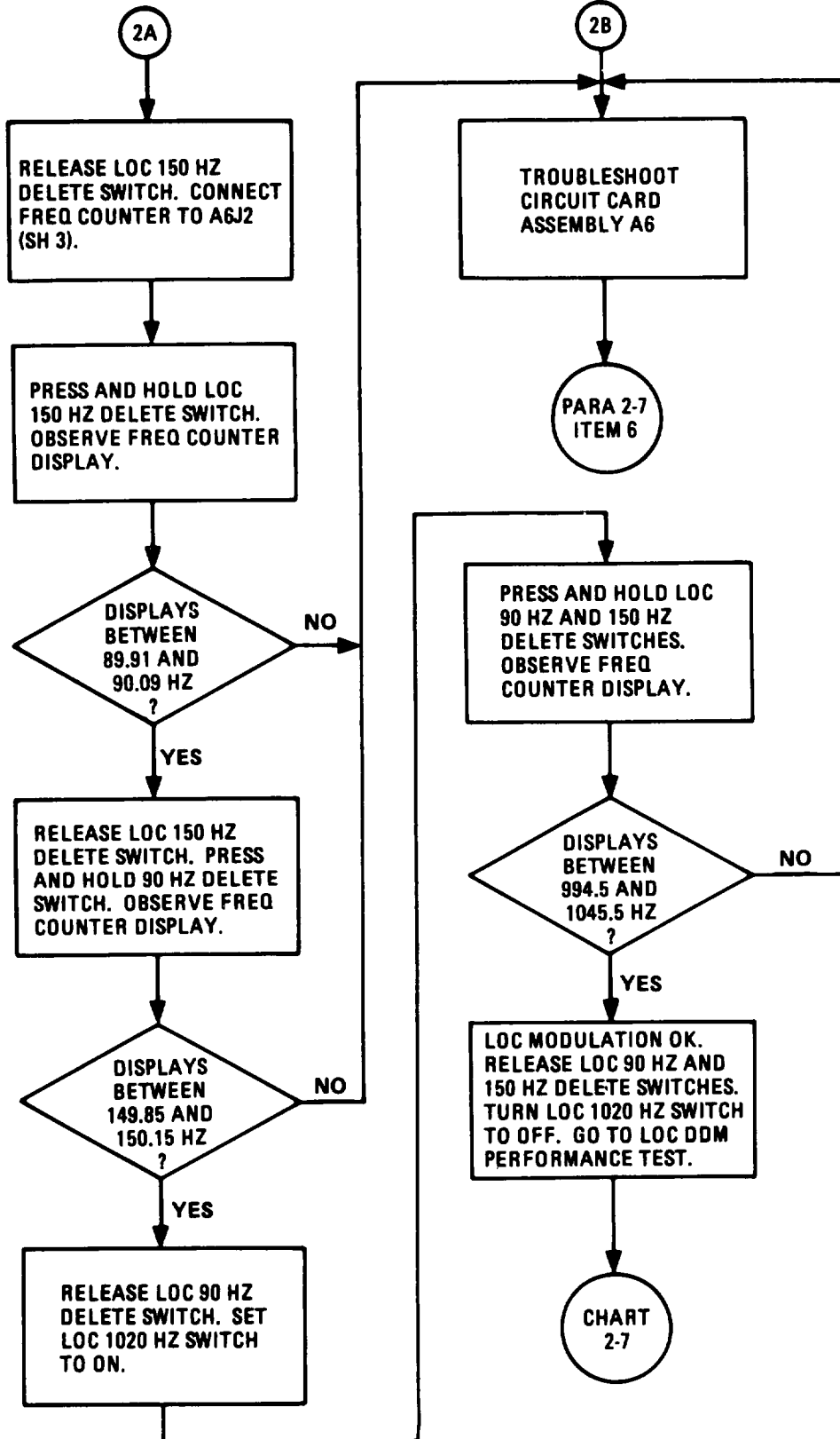
CHART 2-6 LOC Modulation Performance Test (Sheet 2 of 3)
