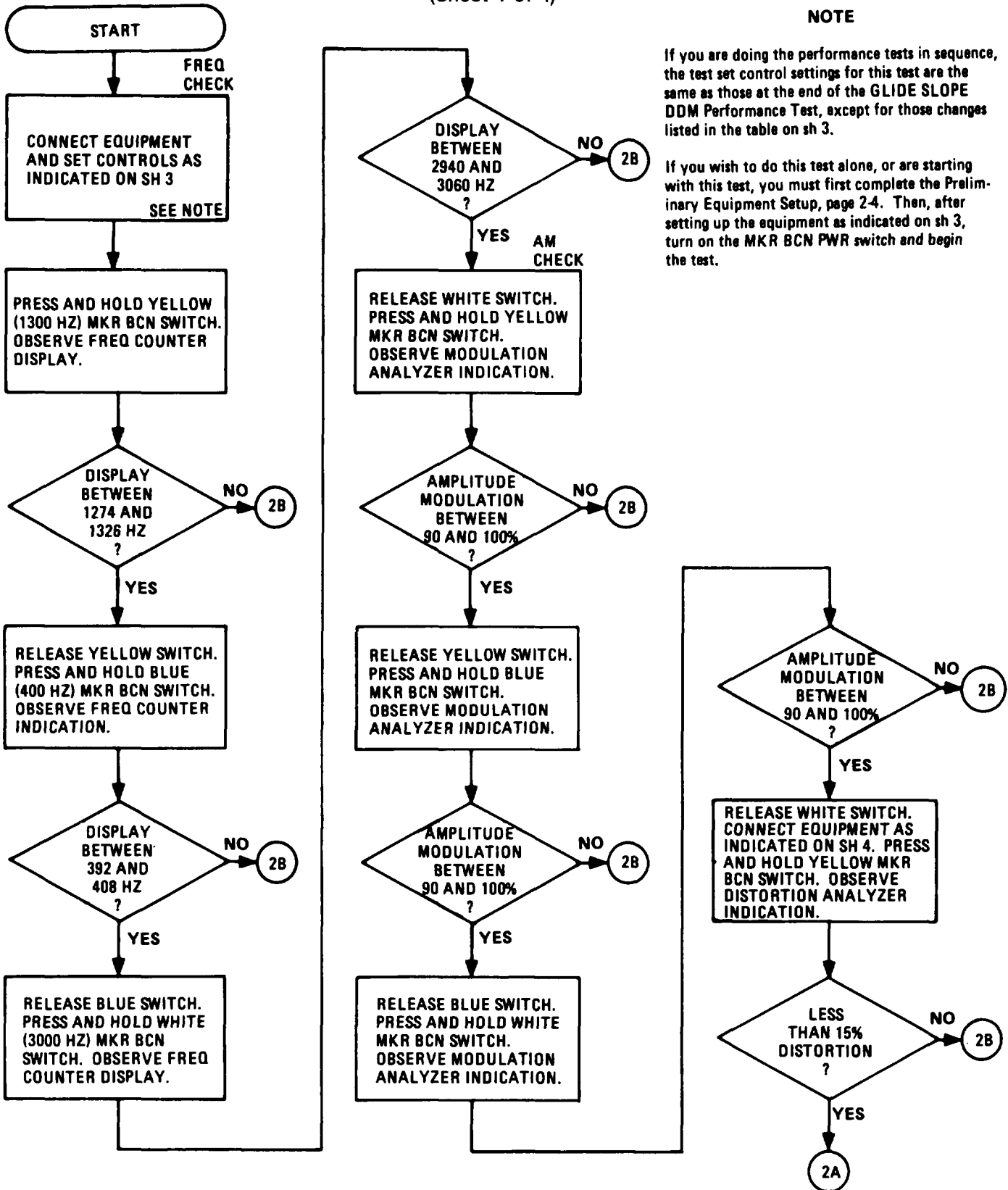
CHART 2-10 Marker Beacon Performance Test (Sheet 1 of 4)
