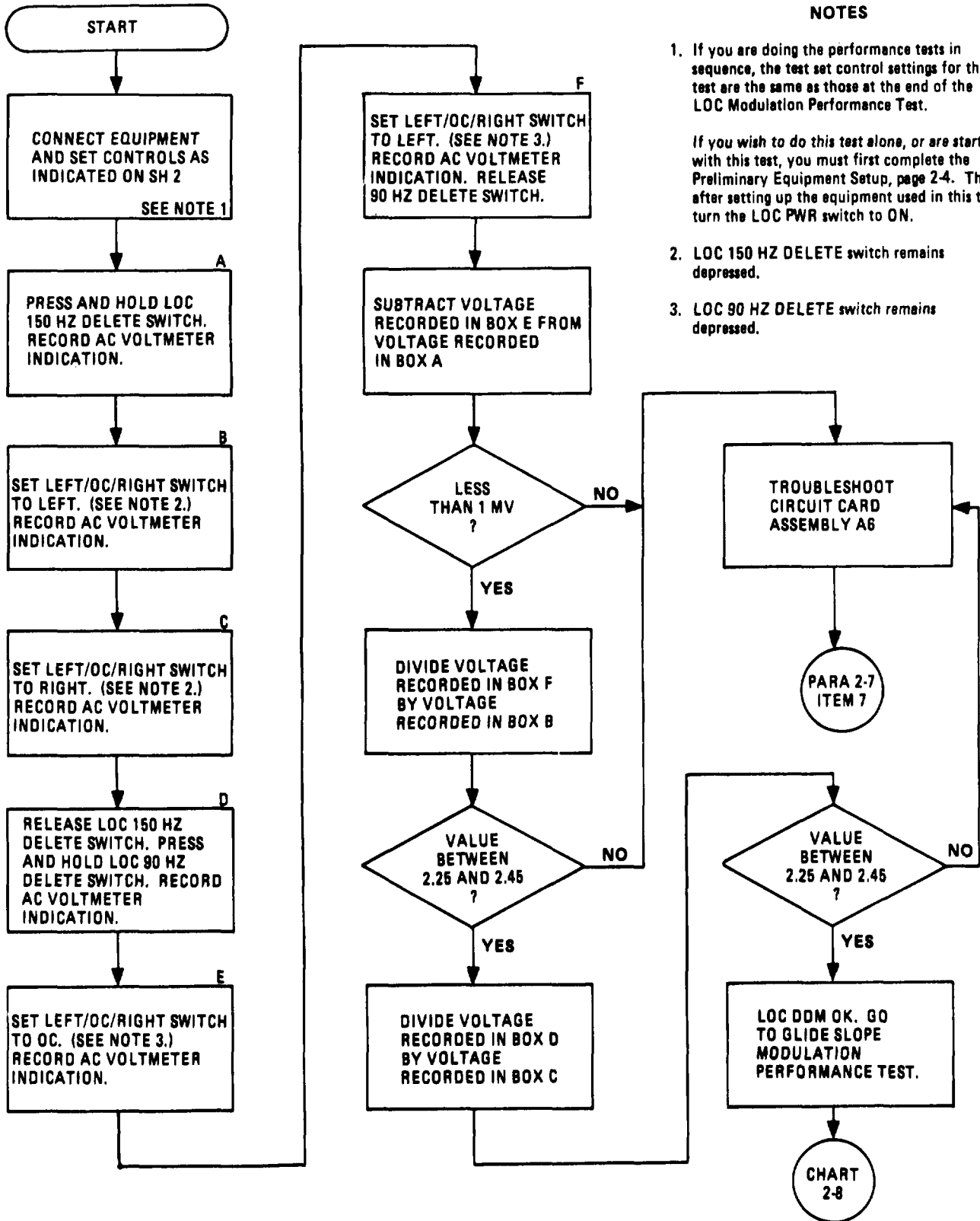
CHART 2-7 LOC DDM Performance Test (Sheet 1 of 2)
