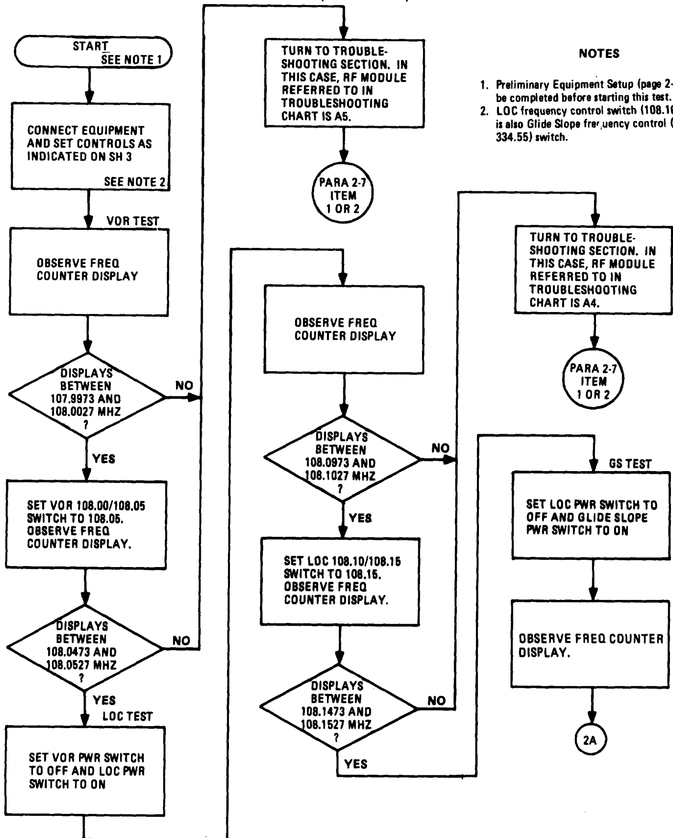
CHART 2-1 Frequency Accuracy Performance Test (Sheet 1 of 3)
